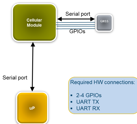
Telit Bundle Solution
