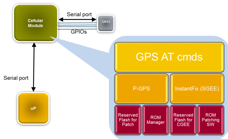
Telit Bundle Solution SW blocks
