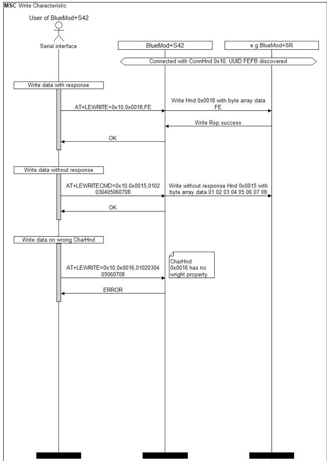
Figure 5: Write characteristic
