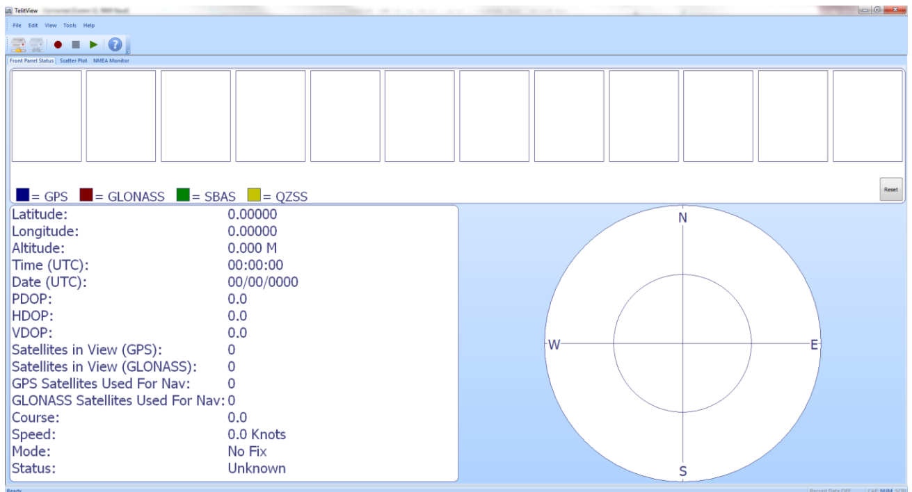
Figure 7 TelitView Application
